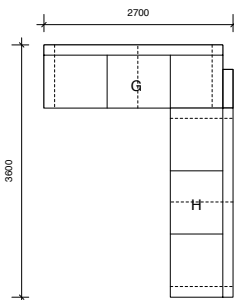
Configuration 7 RHS
