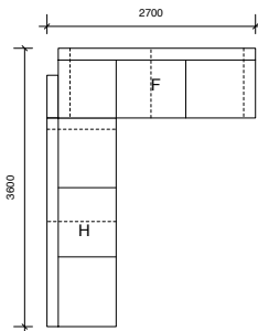
Configuration 7 LHS
